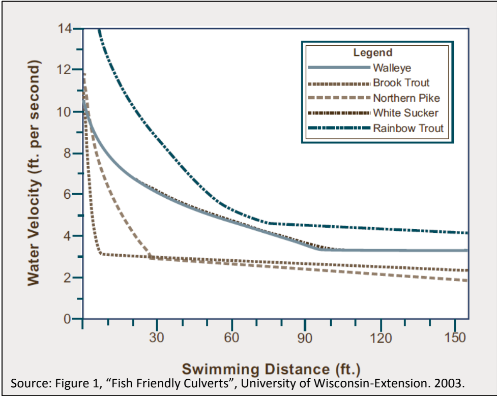
Figure 8: Critical Water Velocities for Fish Passage Design.
