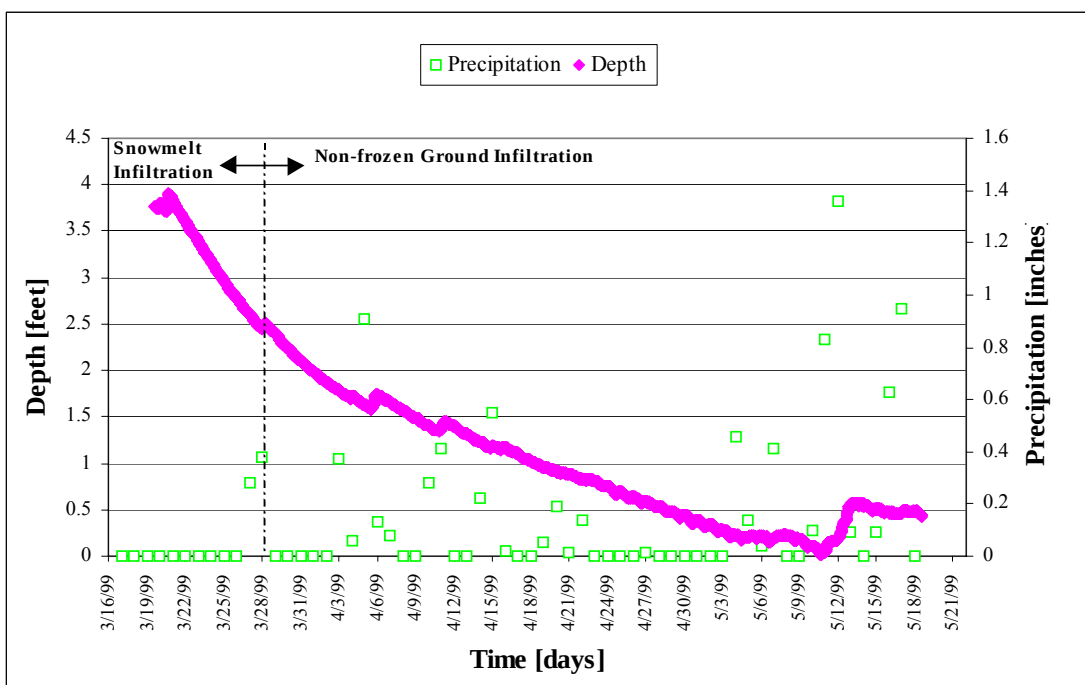
Figure III-9. Depth vs. Time and Precipitation at CD-P50
