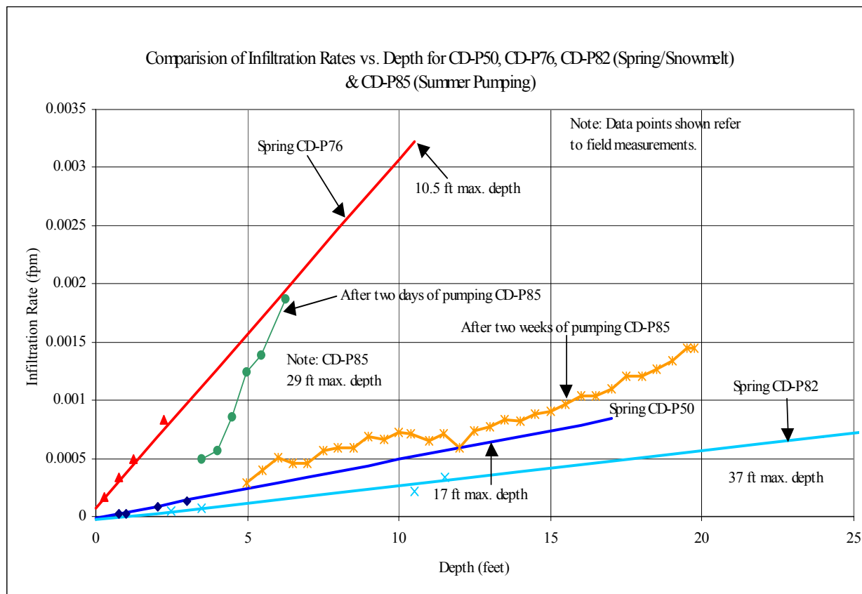
Figure III-16. Linear Regression for Basins used to Calculate Infiltration Rates.
