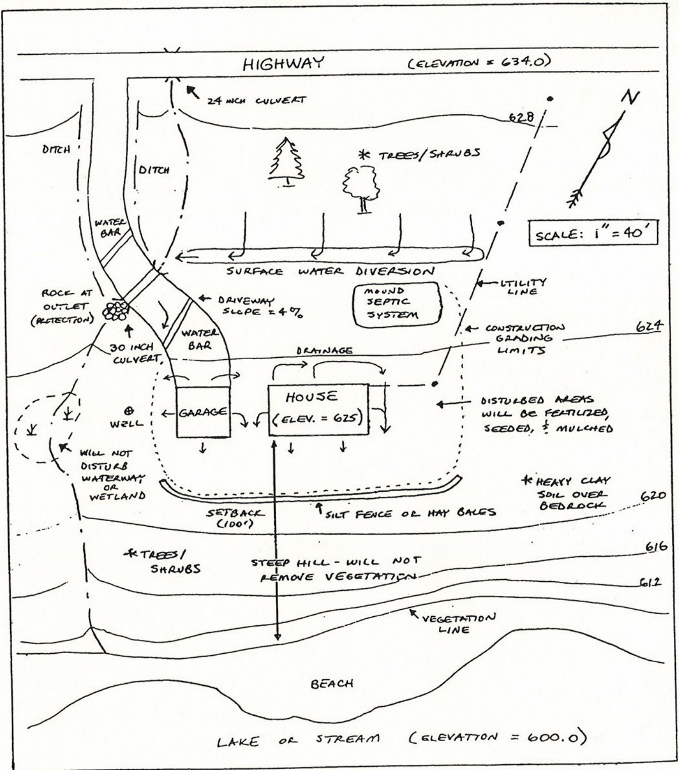
Figure 1: A landscaping plan should include roads, buildings, topography and slope, shoreline, and vegetation.
