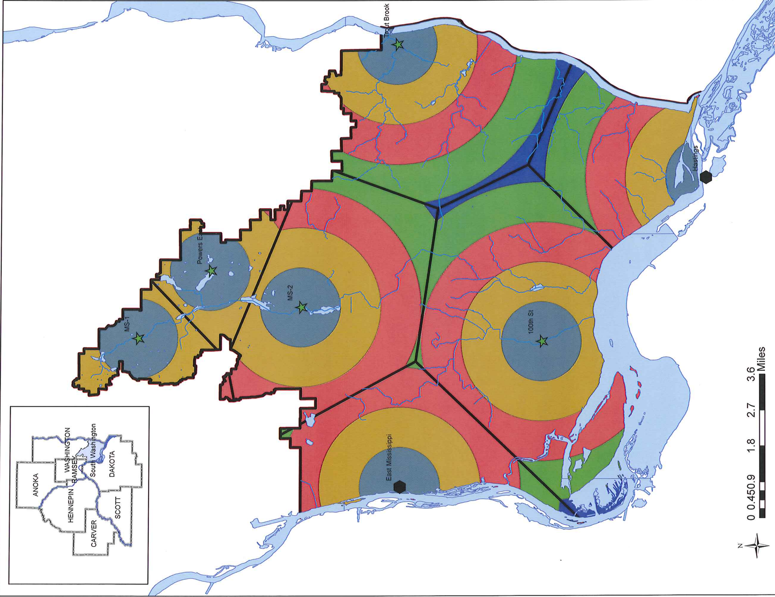
Map 4.1: Precipitation Gauge Sites and Spatial Coverage
