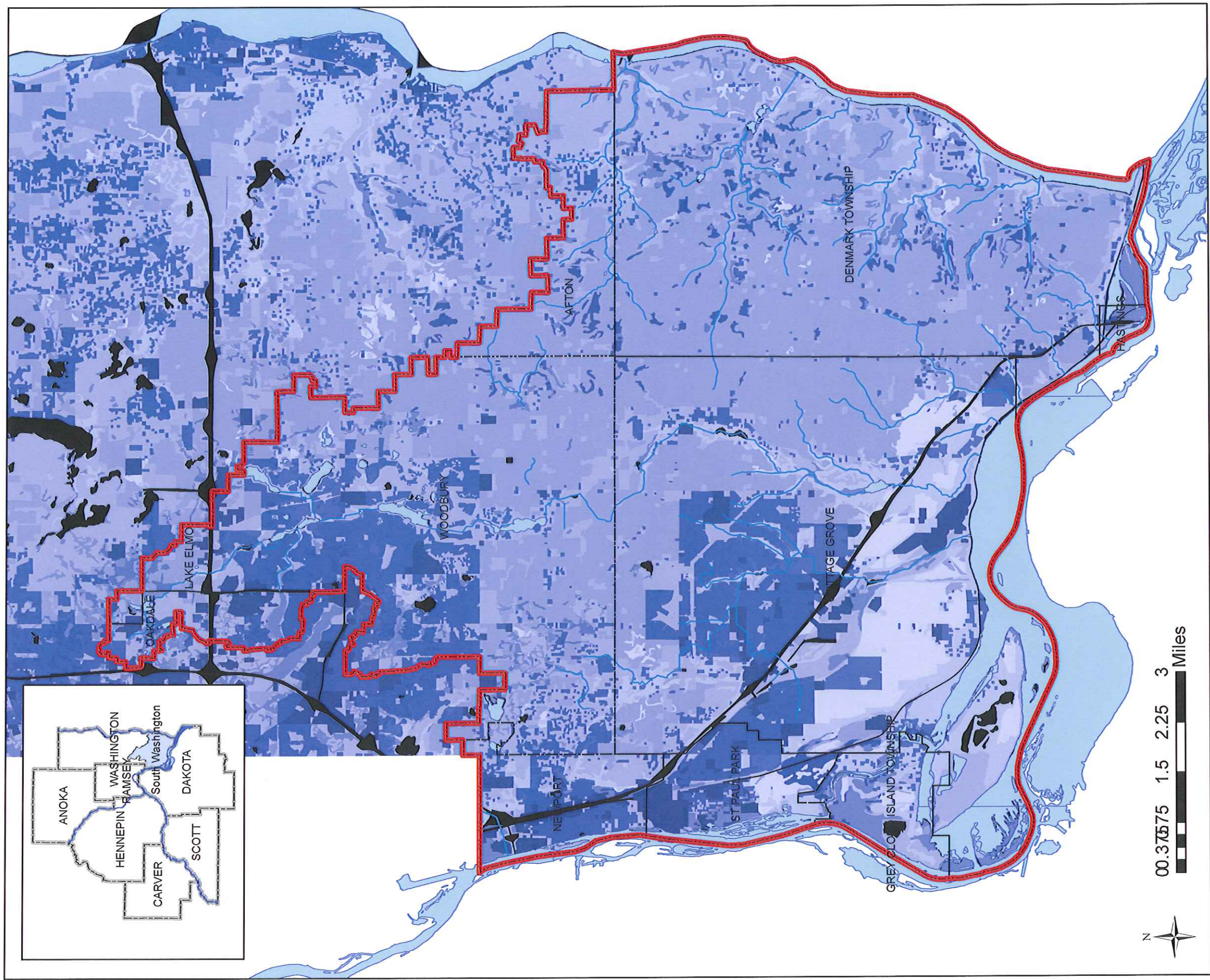
Map 6.2: Estimated Annual Runoff Coefficient for Typical Climatic Conditions
