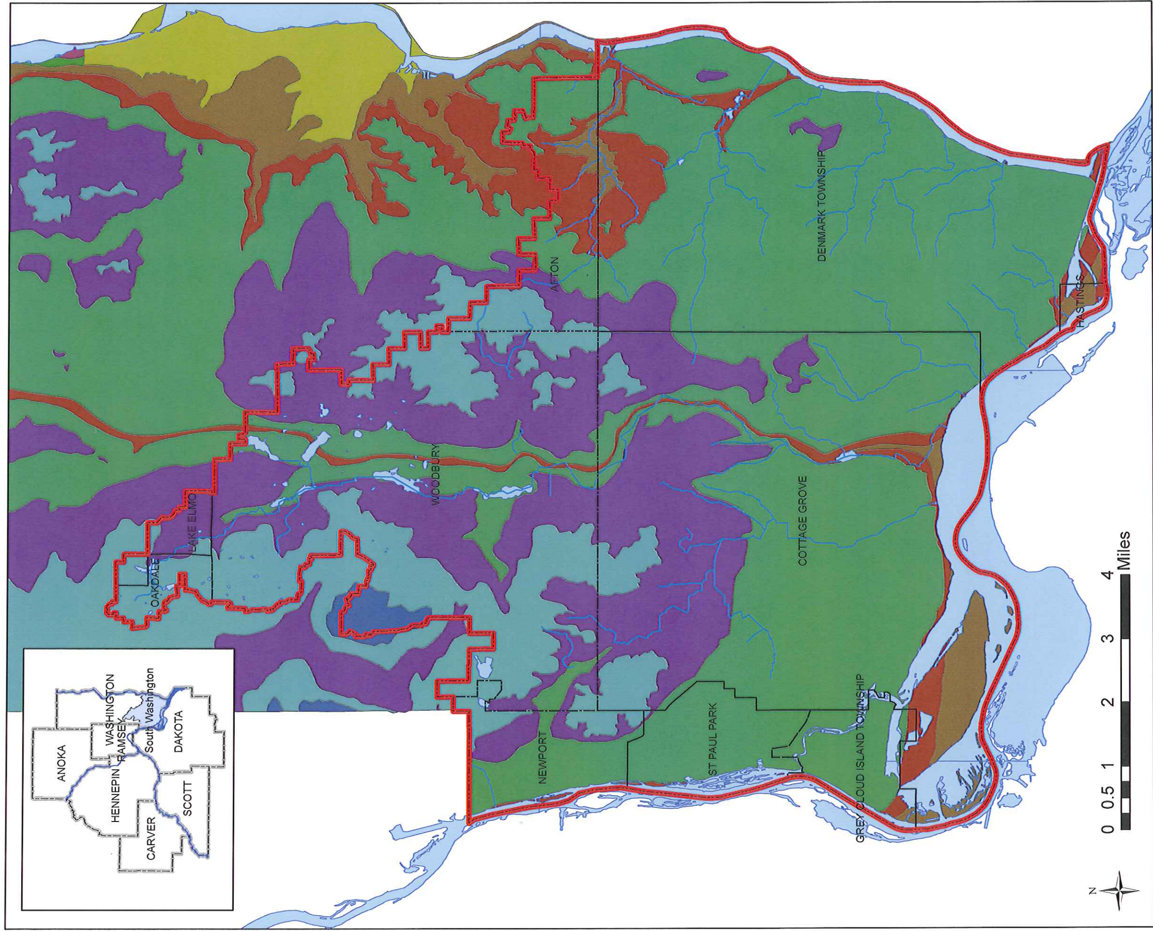
Map 8.4: Bedrock Geology
